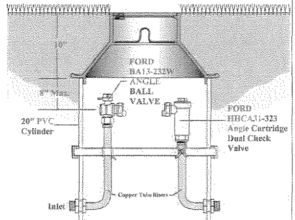
Meter Pit and Setter Detail
